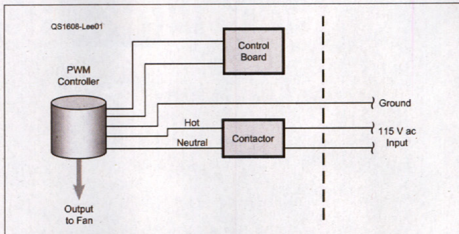
Figure 1 — Block diagram of a heat exchanger fan motor control.
