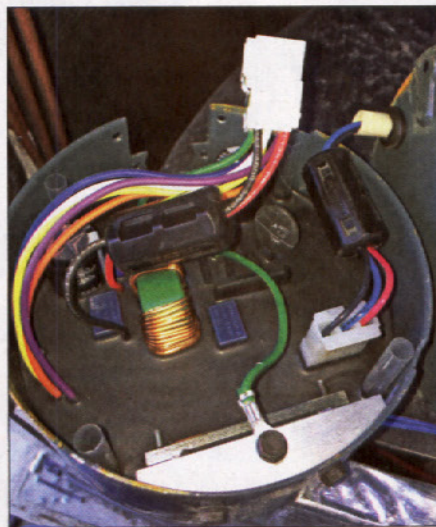
Figure 2 — Interior of the PWM controller shows installed ferrites. [Bob Lee, WØGXA, photo]
