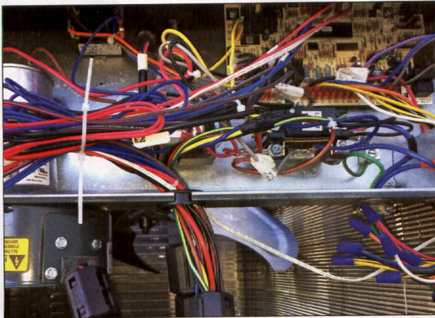
Figure 3 — Wiring harness with ferrites installed. [Bob Lee, W0GXA, photo]
